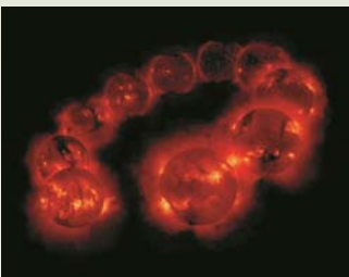
Images of the sun using Montana developed tools for the solar telescopes
